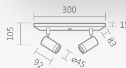
855/2 – spot duplo foco
